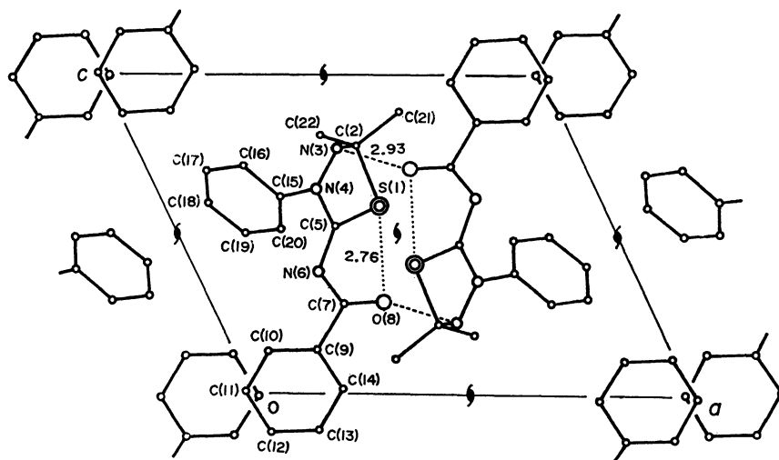
Fig. 2. Crystal structure of 3 viewed along the b axis. Broken lines indicate intermolecular hydrogen bond, and dotted lines S \cdots O interaction (see text). Hydrogen atoms are omitted from the figure for the sake of clarity.
